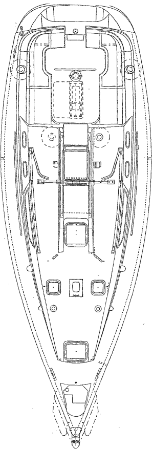
Plan de pont/ Deck layout/ Deckplan
