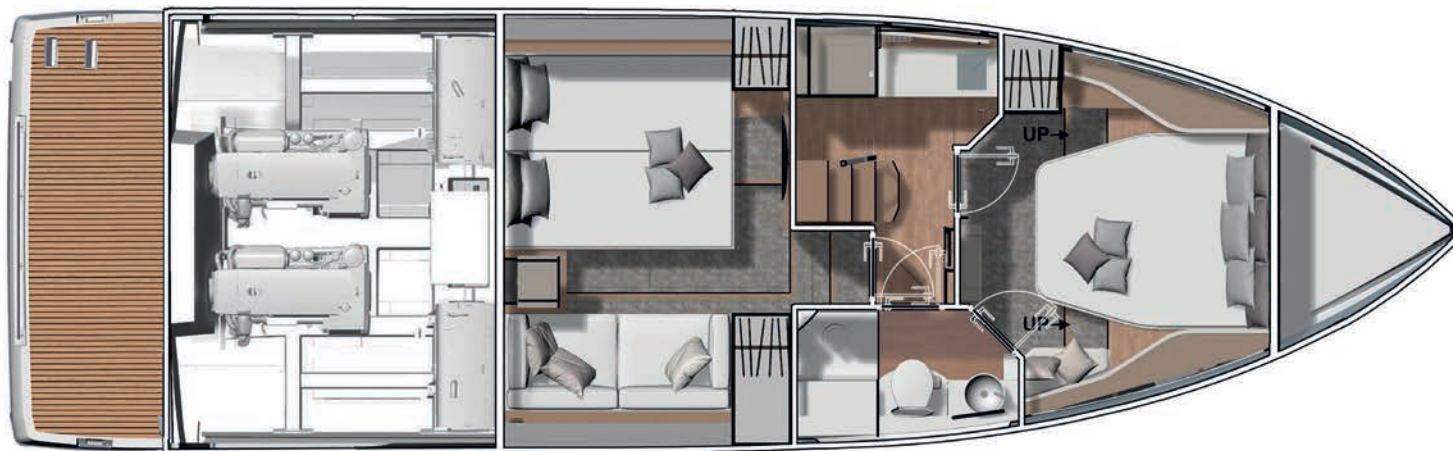
2 cabins, 1 bathroom and 1 breakfast point / Version 2 cabines, 1 salle d'eau et 1 breakfast point
